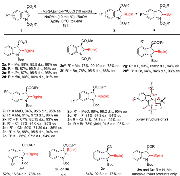
Fig. 2 Substrate scope of reaction. Unless otherwise noted, all the reactions were carried out with 1 (0.2 mmol), (R,R) -QuinoxP* (0.02 mol), CuCl (0.02 mmol), NaOMe (0.02 mmol), t BuOH (0.4 mmol), and B_2pin_2 (0.3 mmol) in toluene (1 mL) at 0 °C for 18 h. The d.r. values ( cis/trans ) were determined by ^1H NMR of crude reaction mixtures. The enantiomeric excesses were determined by chiral HPLC. a The d.r. value was determined by GC of crude reaction mixtures. b The reaction time was 48 hours.
