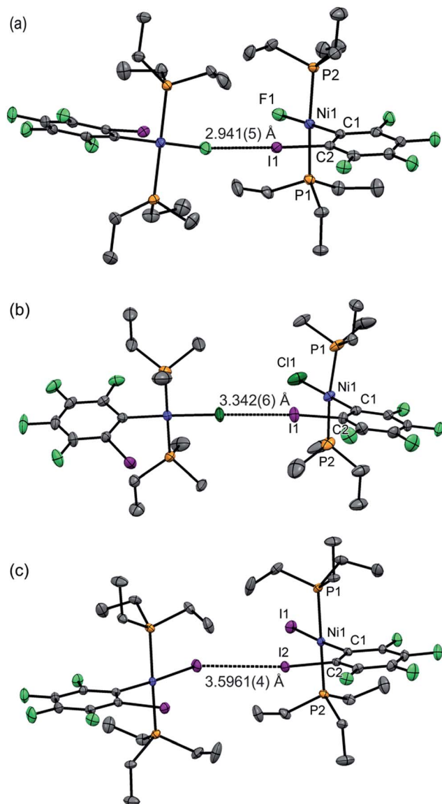
Fig. 3 Molecular structures of 1oX (a) X = F , (b) X = Cl , (c) X = I , showing intermolecular C-I\cdots X-Ni halogen bonds. The structure of 1oCl is disordered (see Table 2). Only the major component is shown. Hydrogen atoms and some methyl groups omitted for clarity. Displacement ellipsoids at 50% probability level. Three-molecule chains are illustrated in the ESI.†
