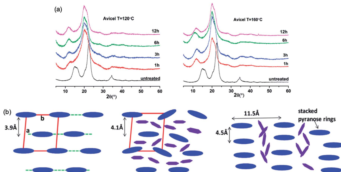
Fig. 6 (a) XRD patterns of Avicel cellulose in [Emim][OAc] at 120 ^\circ\text{C} (left) and 160 ^\circ\text{C} (right). 55 (b) Schematic representation of the arrangement of cellulose crystalline structure (blue) and the intercalated ILs (purple). 56 Reproduced from ref. 55 and 56 with permission from the American Chemical Society.
