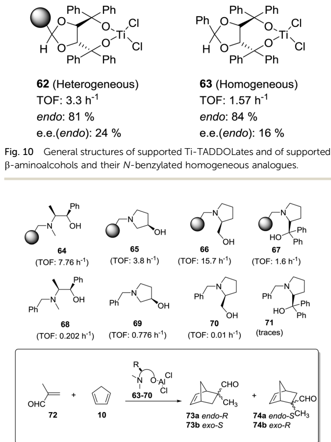
Fig. 11 General structure of supported chiral Lewis acids and the results for their application as catalysts for the Diels–Alder reaction of methacrolein with cyclopentadiene.
