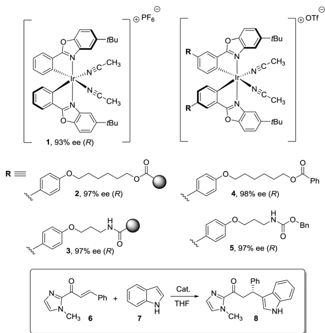
Fig. 1 Effect of structural modification and immobilization on the performance of chiral-at-metal iridium catalysts.
