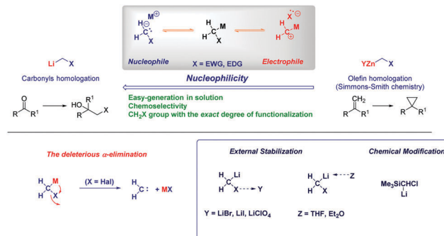
Scheme 1 General features of carbenoids.
