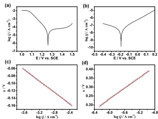
Fig. 2 (a and b) The Tafel curves of a 2 mm-diameter Pt electrode and n-GaAs electrode with area of 0.6 cm 2 in the working solution containing 0.040 mol L -1 \text{KMnO}_4 and 1.84 M \text{H}_2\text{SO}_4 at 35–37 °C. (c and d) The semi-logarithmic relationship between the overpotential and the current for the Pt electrode and n-GaAs electrode.
