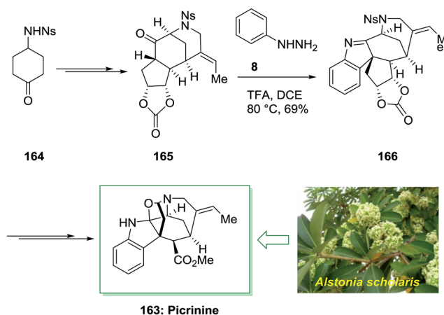
Scheme 33 Total synthesis of picrinine 163 .
