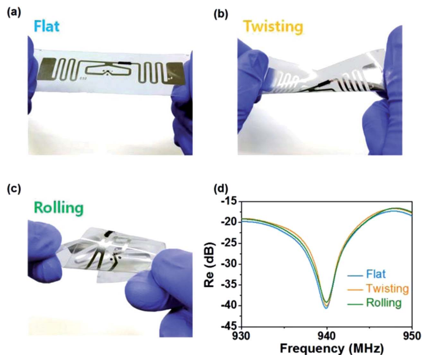
Fig. 8 Photographs of the C-PPy nanparticle-based UHF-RFID tag sensor under different deformation conditions: (a) flat, (b) twisting, and (c) rolling. (d) Normalized reflectance change under flat, twisting, and rolling conditions. [Reprinted with permission from ref. 164 Copyright © American Chemical Society.]
