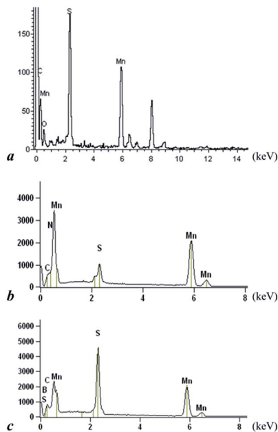
Fig. 5 EDS analysis of (a) MnS/G-9 (b) MnS/NG-9 and (c) MnS/BG-9 nanocomposites.
