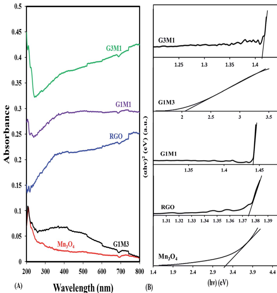
Fig. 4 UV-Vis absorption spectra of RGO, \text{Mn}_3\text{O}_4 , G3M1, G1M1 and G1M3, and their corresponding plots of (\alpha hv)^2 versus (hv) for energy bandgap ( E_g ) determination.
