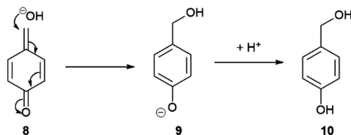
Scheme 3 Proposed formation of 4-hydroxybenzyl alcohol from quinine methide.
