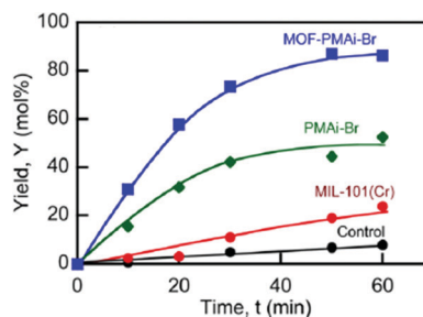
Fig. 17 5-HMF yield (%) from fructose at 100 °C. Conditions: DMSO, 5 mL; D-fructose concentration ( C_{\text{fo}} ), 0.555 mol L -1 ; catalyst loading, 50 mg mL -1 . Control: DMSO solvent with no catalysts added. Reprinted with permission from ref. 122. Copyright 2014, American Chemical Society.
