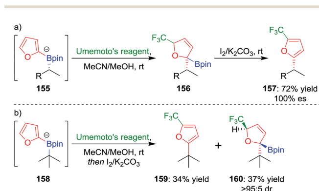
Scheme 21 Transition-metal-free three-component couplings of secondary and tertiary boronic esters with trifluoromethylated furans. R = CH 2 CH 2 C 6 H 4 OMe, Umemoto's reagent = 5-(trifluoromethyl)dibenzothio-phenium trifluoromethanesulfonate.
