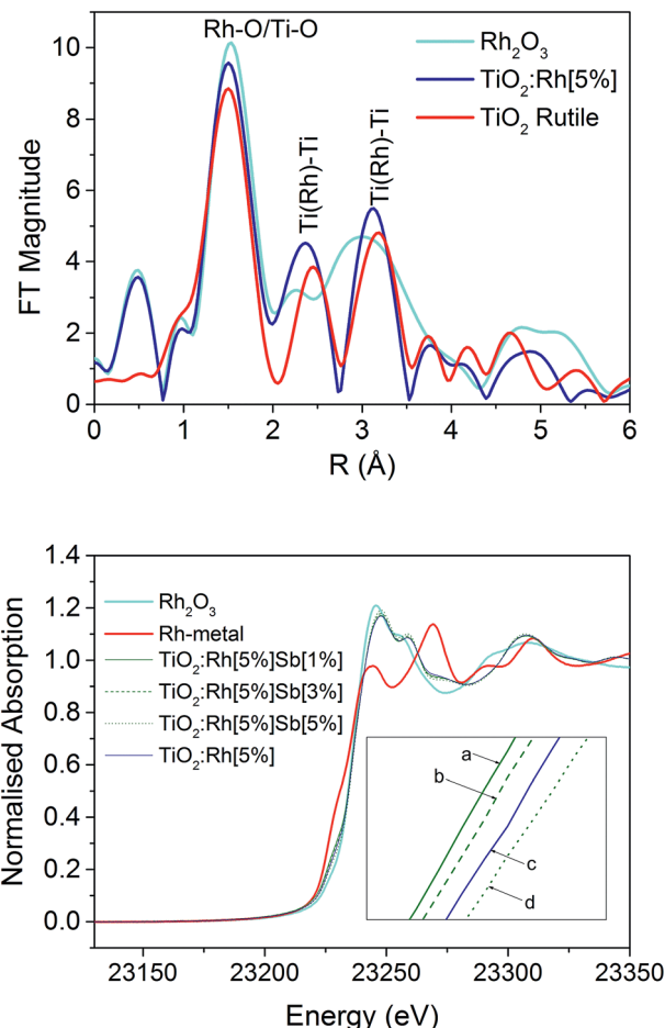
Fig. 1 Fourier transform of the Rh K-edge EXAFS of TiO 2 :Rh[5%] by comparison with TiO 2 (Ti K-edge EXAFS) and Rh 2 O 3 (Rh K-edge EXAFS) standard powders (top), and Rh K-edge XANES of Rh 2 O 3 , Rh-metal, TiO 2 :Rh[5%], TiO 2 :Rh[5%]Sb[1%], TiO 2 :Rh[5%]Sb[3%] and TiO 2 :Rh[5%]Sb[5%] (bottom); note that the Fourier transform presented here are not phase shift corrected and therefore the distances appear shorter than expected values. Actual distances reported here are based on the full analysis of the EXAFS data which includes phase shift correction.
