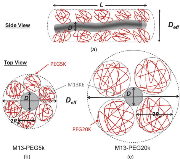
Fig. 1 (a) Schematic representation of the M13KE semi-flexible rod-like virus sterically stabilized with a grafted layer of the hydrophilic PEG polymer. (b and c) The top views have been drawn to scale considering both the bare diameter of the rod-like virus D , and the corresponding radius of gyration R_g of the PEG polymer with molar weights of 5k and 20k Da, respectively. The geometrical effective diameter D_{\text{eff}} \approx D + 4R_g is indicated by a dashed line.
