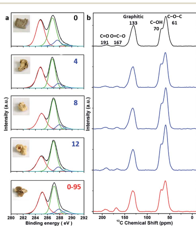
Fig. 1 (a) C 1s XPS spectra and photographs (inset), and (b) magic-angle spinning 13 C ssNMR spectra of different freeze-dried GO- n and GO-0-95 samples; the values of n are depicted in (a).
