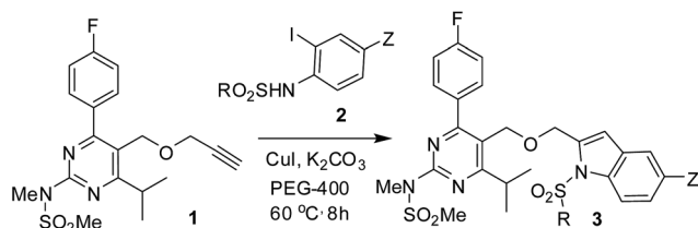
Scheme 2 Cu-Catalyzed \text{Pd} /ligand-free synthesis of rosvastatin based indole derivatives in PEG-400.
