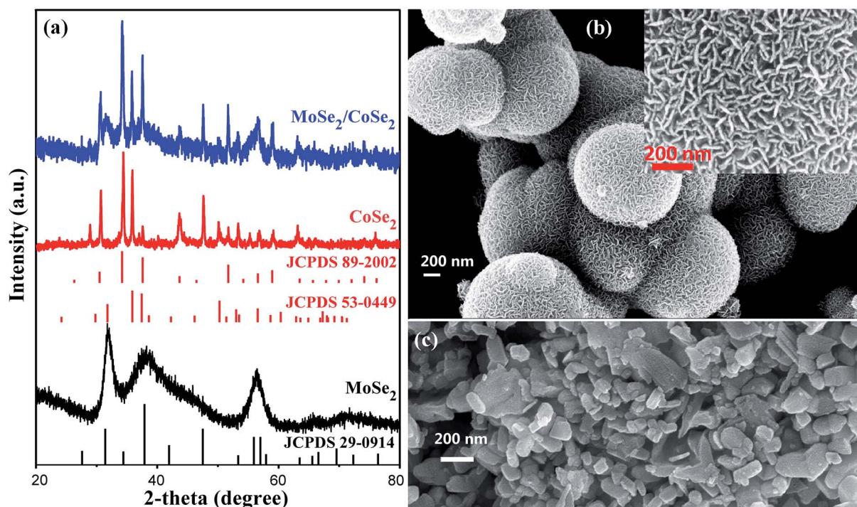
Fig. 1 (a) XRD patterns of the as-synthesized pure \text{MoSe}_2 , \text{CoSe}_2 , and \text{MoSe}_2/\text{CoSe}_2 composite; (b) and (c) are SEM images of the as-synthesized pure \text{MoSe}_2 and \text{CoSe}_2 , respectively.
