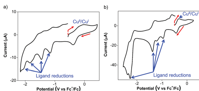
Fig. 3 Cyclic voltammograms of (a) 1.0 mM of 3 and (b) 1.0 mM of 4 in DMF/DMSO 1 : 1 (v : v), with 0.10 M n\text{-Bu}_4\text{NBARF}_4 as the electrolyte, each at a scan rate of 100\text{ mV s}^{-1} with its scan direction and initial potential indicated by the red arrows and red vertical dashed line respectively. The data are reported relative to \text{Fc}^+/\text{Fc} .
