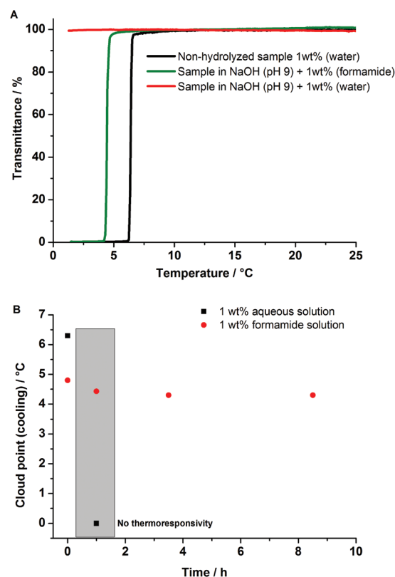
Fig. 7 (A) Hydrolysis stability of poly(AAm 87 -co-AN 12 ) in NaOH (pH 9), with and without sacrificial additives. (B) Stability of the thermoresponsive behavior in aqueous media of poly(AAm 87 -co-AN 12 ) at 85 °C depending on time, with and without sacrificial additives.
