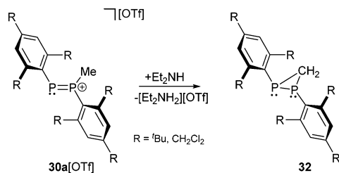
Scheme 11 Formation of diposphirane 32 by deprotonation of 30a[OTf] .
