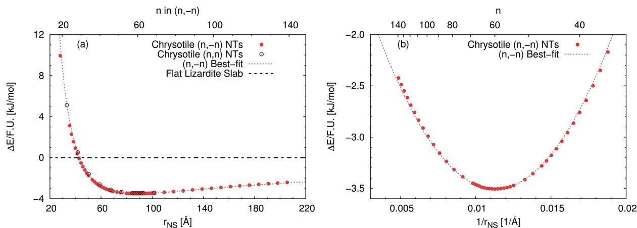
Fig. 3 Energy difference per formula unit of (n, -n) single-walled chrysotile nanotubes with respect to the flat lizardite slab [\text{kJ mol}^{-1}] , as a function of (a) NS radius [\text{\AA}] and index n , and (b) inverse NS radius [\text{\AA}^{-1}] and index n . The superimposed curve has been obtained through quadratic best-fit over a set of 16 points around the energy minimum. In (a), data for the (n, n) series are also shown. In (b), only the subset of (n, -n) data in the energy range of -3.6 – -2 \text{ kJ mol}^{-1} is shown. All the corresponding (n, -n) data are reported in Table S1 in the ESI.†
