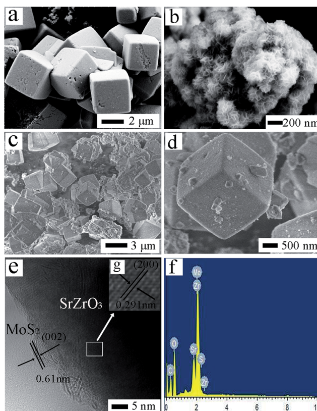
Fig. 3 (a) SEM images of SrZrO 3 , (b) SEM images of MoS 2 , (c and d) SEM images of SM8, (e and g) HRTEM images of SM8, (f) EDX pattern of SM8 photocatalyst in (c).
