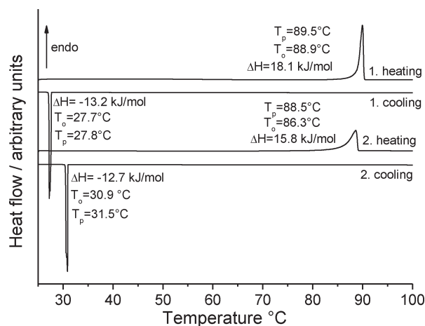
Fig. 9 DSC heating and cooling curves for form 1t at 1 °C min −1 ; the peak ( T p ) and onset ( T o ) temperatures are given in °C and the enthalpy Δ H in kJ mol −1 .
