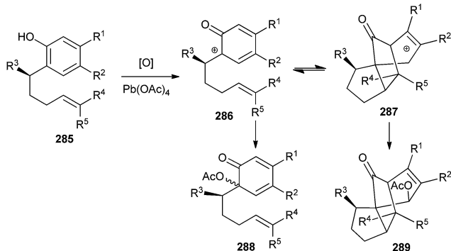
Scheme 61 Intramolecular [5 + 2] cycloaddition of phenoxonium intermediates.
