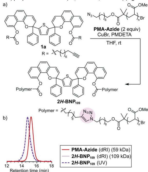
Figure 1. (a) Synthesis of a poly(methyl acrylate) polymer (109 kDa, \mathcal{D} = 1.17 ) containing a chain-centered 2H -bis-naphthopyran mechanophore unit via CuAAC. (b) Characterization by GPC-MALS with differential refractive index (dRI) and in-line UV detection (345 nm) confirms 2H -bis-naphthopyran functionalization near the chain center.
