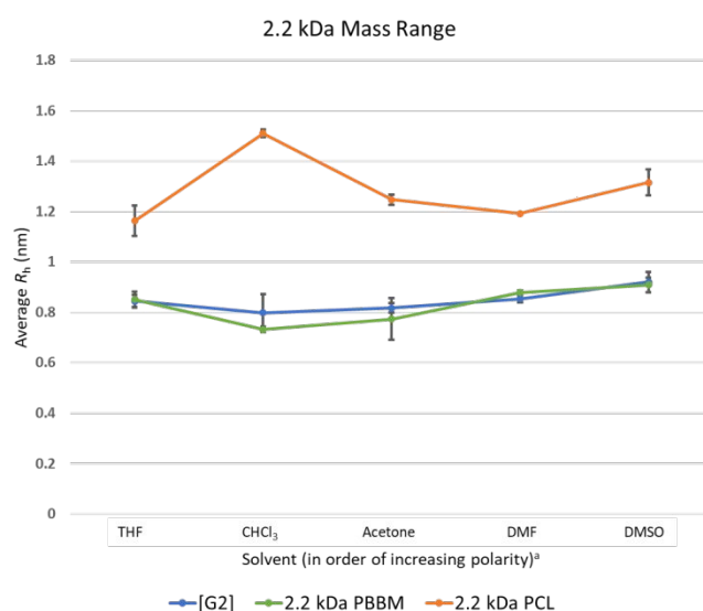
Fig. 6 Calculated average R_h values, from DOSY- 1 H NMR, for Tetra[G2]Bnz 8 , 2.2 kDa PCL, and 2.2 kDa PBBM in all tested solvents.
