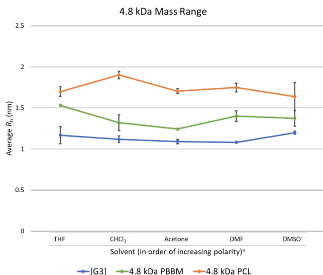
Fig. 7 Calculated average R_h values, from DOSY- 1 H NMR, for Tetra[G3]Bnz 16 , 4.8 kDa PCL, and 4.8 kDa PBBM in all tested solvents.
