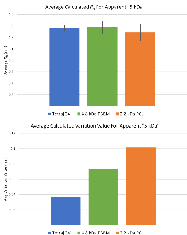
Fig. 9 Average R_h and variation values for apparent 5 kDa Tetra[G4]Bnz 32 , 4.8 kDa PBBM, and 2.2 kDa PCL.
