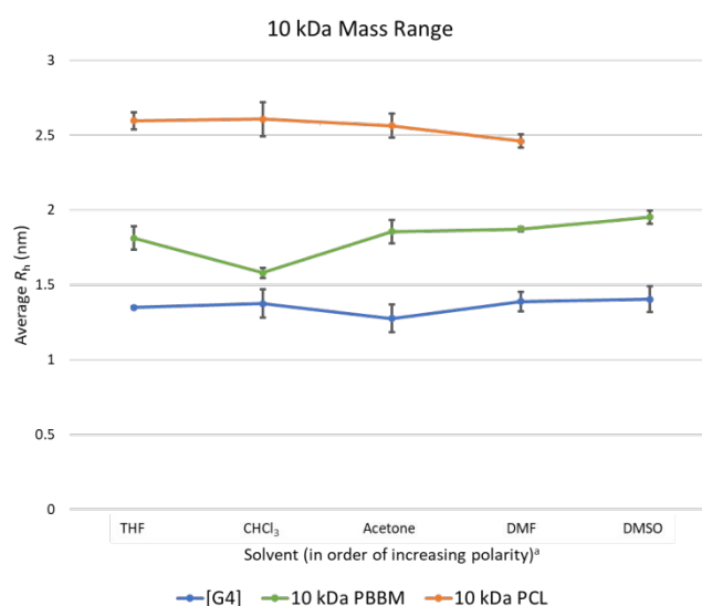
Fig. 8 Calculated average R_h values, from DOSY- 1 H NMR, for Tetra[G4]Bnz 32 , 10 kDa PCL, and 10 kDa PBBM in all tested solvents.
