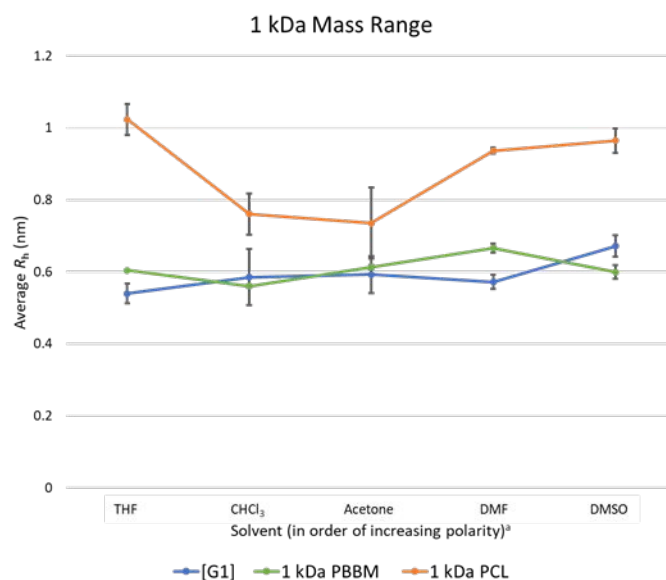
Fig. 5 Calculated average R_h values, from DOSY- ^1\text{H} NMR, for Tetra[G1]Bnz 4 , 1 kDa PCL, and 1 kDa PBBM in all tested solvents.
