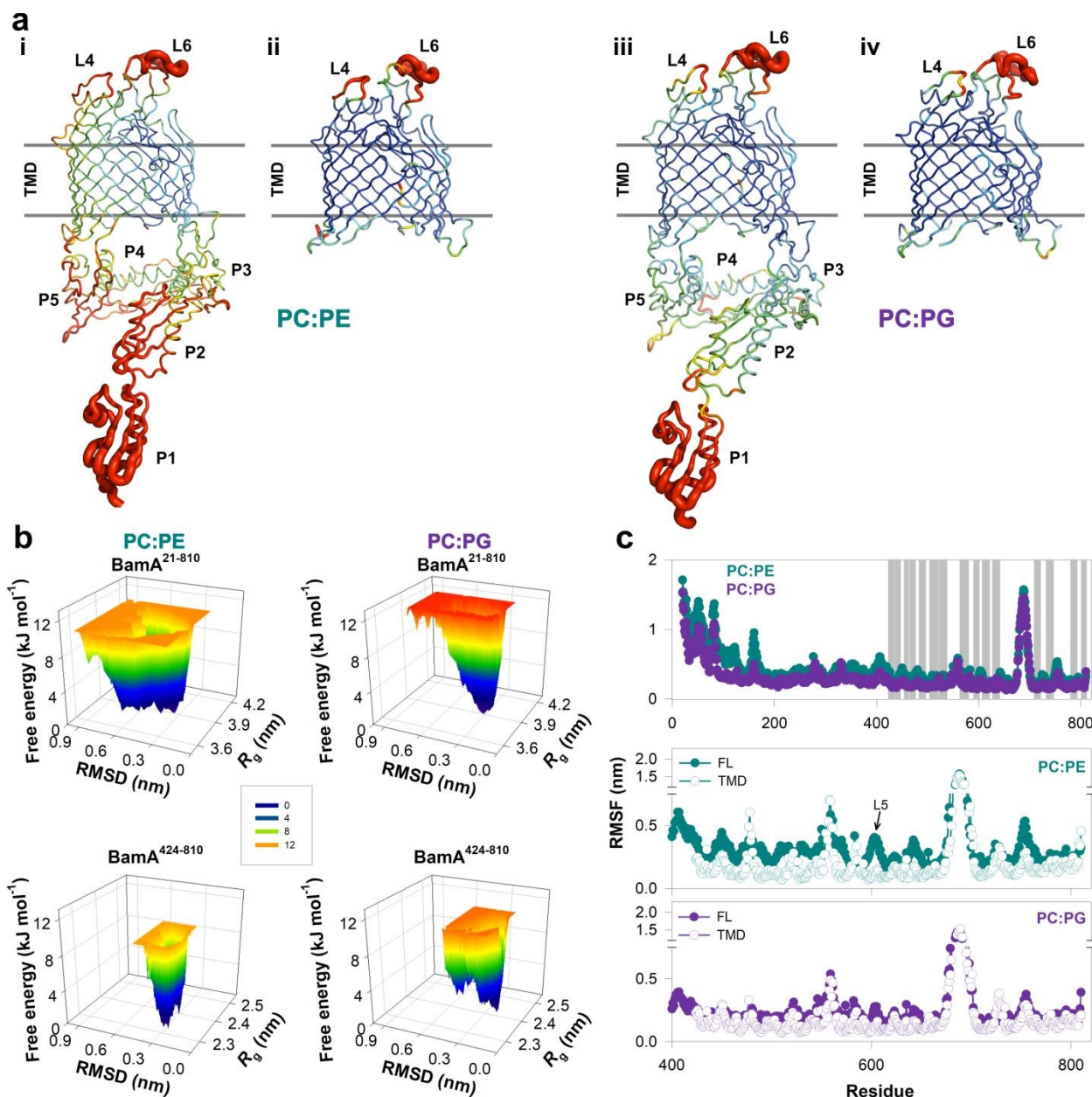
Figure 4: Bama β-barrel dynamics are regulated by the membrane composition and POTRA. (a) Results of all-atom MD simulations of full-length Bama and POTRA - Bama in PC:PE and PC:PG membranes. Atomic displacement (B-factor analysis) is rendered as sausage representation (red, highest RMSD; dark blue, lowest RMSD). In PC:PE (a,i), POTRA, L4, and L6 exhibit high structural dynamicity, which allosterically translates to increased dynamicity of N-terminal β3–β6. POTRA deletion abolishes this plasticity in the TMD (a,ii), limiting the conformational flexibility to L4 and L6. In contrast, PC:PG membranes restricts the conformational dynamicity to only POTRA1 in full-length Bama (a,iii) and additionally L6 (a,iii and a,iv). PE increases Bama TMD and POTRA plasticity, while the TMD is conformationally rigid in PG, irrespective of POTRA. (b, top panels) Free energy landscape (FEL) of full-length Bama (residues 21-810) show marked difference in the presence of PC:PE (top left) and PC:PG (top right). Full-length Bama displays greater conformational freedom in PC:PE (higher RMSD; broader FEL profile) than PC:PG. A narrower FEL profile suggests that PC:PG restricts the β-
