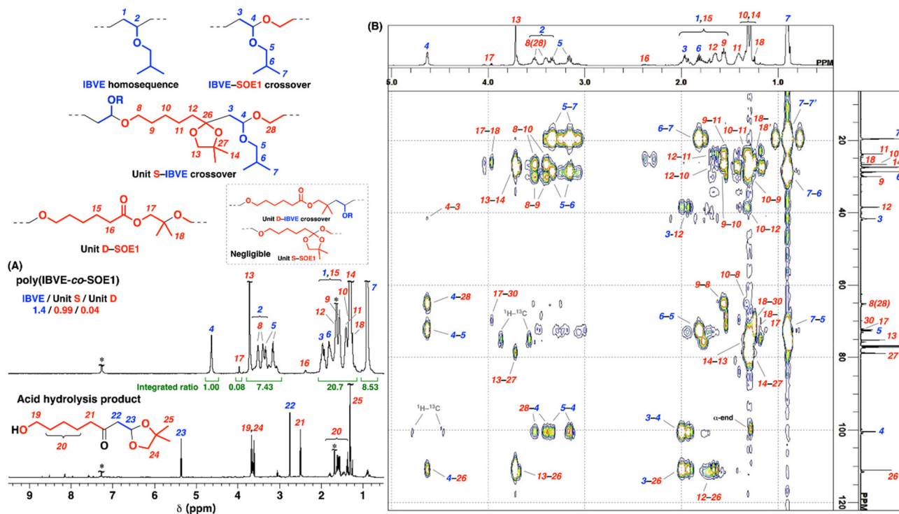
Fig. 2 (A) 1 H NMR spectra of poly(IBVE- co -SOE1) (upper; entry 5 in Table 1; after purification by reprecipitation in methanol, a pink curve in Figure 1B) and acid hydrolysis product (lower). (B) 1 H- 13 C HMBC NMR spectrum of poly(IBVE- co -SOE1) (entry 9 in Table 1; a limited region of the spectrum is shown; see Fig. S9 for a wider region). See the footnote of Table 1 for the polymerization conditions. In CDCl 3 at 30 °C. *CHCl 3 or water.
