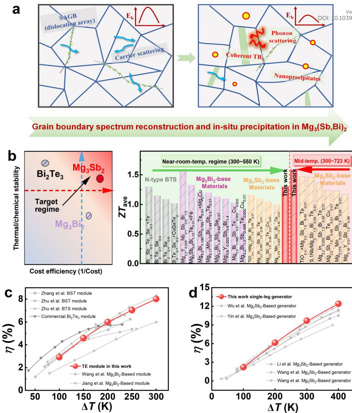
Figure 1 The schematic of the main mechanism and superior thermoelectric performance in \text{Mg}_3(\text{Sb}, \text{Bi})_2 -based materials. a Schematic diagram of a strain-mediated grain-boundary spectrum reconstruction and the dispersed in-situ nanoprecipitates. b Raw-material cost and stability comparison, and the comparison of the average ZT values of this work with state-of-the-art n-type \text{Bi}_2\text{Te}_3 -, \text{Mg}_3\text{Bi}_2 -, and \text{Mg}_3\text{Sb}_2 -based TE materials at different temperature ranges. [33, 44–60] c The comparison of conversion efficiency of TE module in this work paired with a p-type \text{MgAgSb} material and previously reported \text{Bi}_2\text{Te}_3 - and \text{Mg}_3\text{Bi}_2 -based modules. [44, 57, 61–64] d The efficiency comparison between the single-leg generator and other \text{Mg}_3\text{Sb}_2 -based systems. [57, 60, 65–68]
