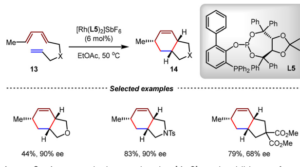
Scheme 8 Asymmetric intramolecular [4+2] cycloadditions of unactivated trienes catalyzed by a rhodium(I)/TADDOL-derived phosphine-phosphite ligand complex.
