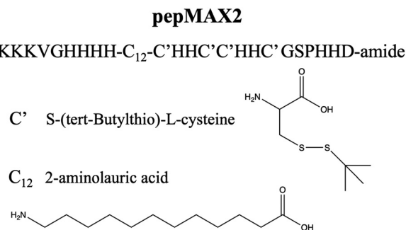
Fig. 1 The chemical structure of pepMAX2.
