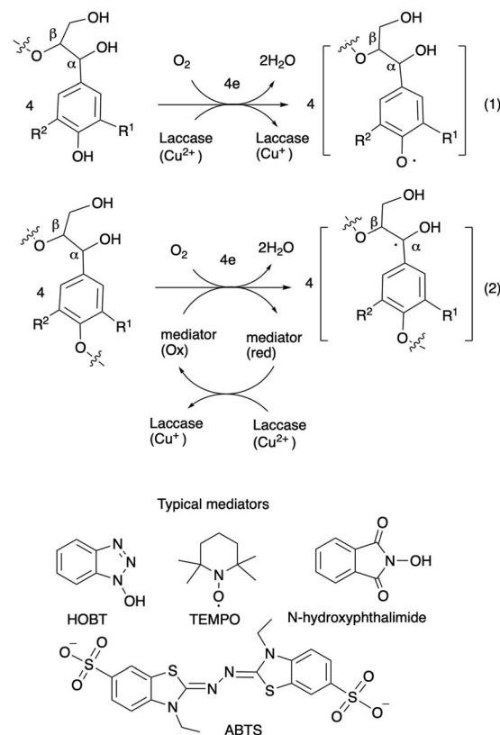
Fig. 3 Laccase-mediated oxidation. 17,29,76–78
