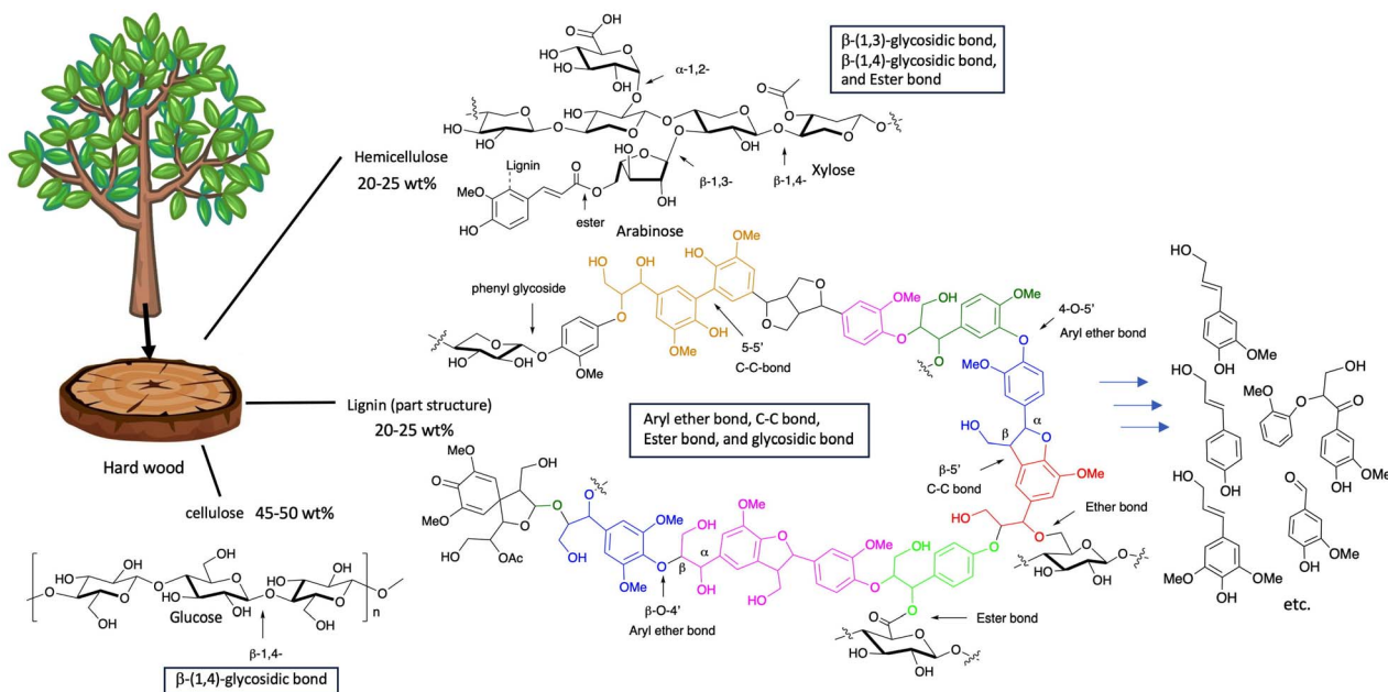
Fig. 1 Schematic image of the "structure model of the core part of lignocellulose". 4-12 The tree image was obtained from the following site: https://tegakisoai.com/archives/29099#google_vignette (accessed 17th February 2025).
