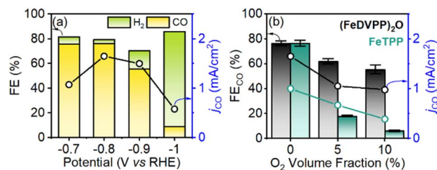
Fig. 5 (a) Faradaic efficiency (FE) and CO partial current density ( j_{\text{CO}} ) of heterogenized ( FeDVPP ) 2 O on the CNT/CP electrode in CO 2 -saturated 0.5 M KHCO 3 after 30 min of electrolysis at different potentials. (b) Comparison of performance of ( FeDVPP ) 2 O and FeTPP after 30 min of electrolysis at -0.8 V vs. RHE at different O 2 volume fractions (in the CO 2 + O 2 mixture).
