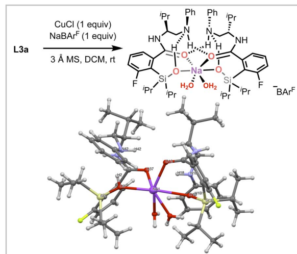
Fig. 4 Single-crystal structure of intermediate complex [( L3a ) 2 /Na·(H 2 O) 2 ] + [BAR F ] - isolated from slow solvent evaporation over two months. The BAR F anion has been omitted for clarity. Selected bond distances (Å), H-bonding interactions, and angles (deg): Si(2)-O(2): 1.634(4), Na(1)-O(2): 2.284(10), Na(1)-O(37): 2.441(8), O(2)-H(2)...N(42), N(18)-H(18)...O(37), N(42)-H(42)...O(13), O(1B)-H(1B1)...N(18), ∠ Si(2)-O(2)-Na(1): 133.7(2).
