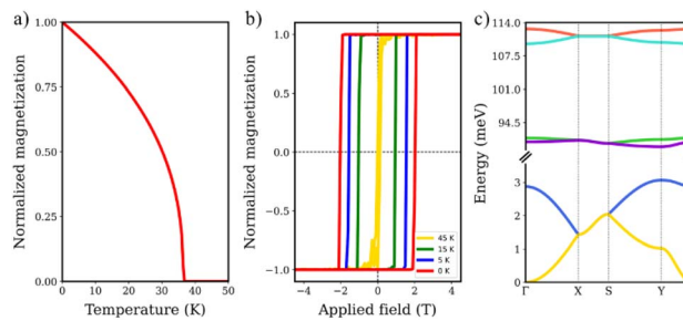
Fig. 4 Simulated (a) Curie temperature, (b) hysteresis loop at different temperatures and (c) magnon dispersion for the V_3N@C_{80} graphenodofullerene network.
