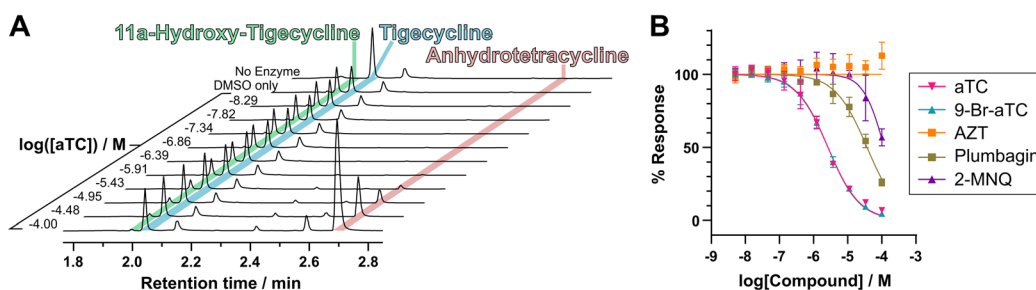
Fig. 5 A novel chromatography-based activity assay allows measurement of IC_{50} values with reduced interference from UV-active compounds. (A) UPLC chromatograms demonstrating dose-dependent inhibition of Tet(X4) using known inhibitor anhydrotetracycline as an example. Chromatograms show the absorbance at 254 nm in arbitrary units. (B) Dose–response curves for inhibition of Tet(X4) activity, monitored by UPLC peak integrals to calculate turnover, with previously reported inhibitors. 33,38,39 Conditions were: 20 \mu M tigecycline, 50 nM Tet(X4), 10 \mu M FAD, 5 mM MgCl_2 and 100 \mu M NADPH in 100 mM TAPS buffer (pH 8.5) with a final concentration of 1% v/v DMSO.
