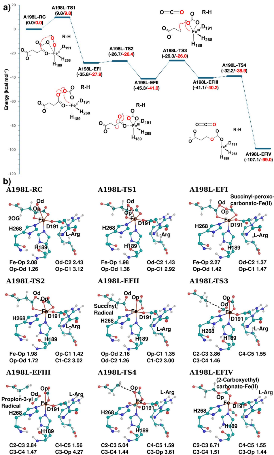
Fig. 7 (a) Reaction profile of the \text{O}_2 activation mechanism in the A198L-EFE variant. Relative energies are given in \text{kcal mol}^{-1} at QM(B2)/MM (black) and QM(B3)/MM (red) levels. The profile was plotted at the QM(B3)/MM level. (b) Optimized structures obtained during the QM/MM simulations. Distances are mentioned in Å.
