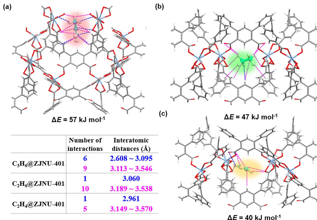
Fig. 3 Calculation of the optimized adsorption sites for (a) \text{C}_3\text{H}_6 and (b) \text{C}_2\text{H}_6 and (c) \text{C}_2\text{H}_4 within ZJNU-401, and comparison of the host–guest interactions among them.
