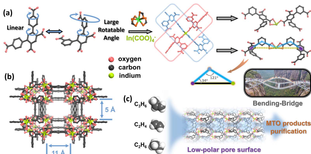
Fig. 1 Structural description of ZJNU-401: (a) from the "bending-bridge" design of the ligand to the assembly with mononuclear \text{In}^{3+} to form the 4-c node; (b) 1D pore channel of ZJNU-401; (c) low-polarity pore surface for effective MTO product purification.
