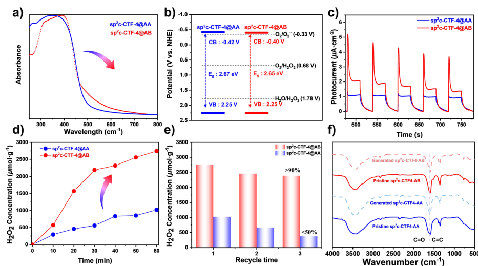
Fig. 3 (a) UV-vis DRS of sp 2 c-CTF-4@AA and sp 2 c-CTF-4@AB. (b) Band structures of sp 2 c-CTF-4@AA and sp 2 c-CTF-4@AB. (c) Chopped photocurrent density vs. time recorded on sp 2 c-CTF-4@AA and sp 2 c-CTF-4@AB at 0.6 V vs. RHE. (d) Time-dependent H 2 O 2 photogeneration using visible light for sp 2 c-CTF-4@AA and sp 2 c-CTF-4@AB (5 mg catalyst in 10 mL pure water); (e) recycling H 2 O 2 production on sp 2 c-CTF-4 (reaction time: 1 h); (f) FTIR spectra of sp 2 c-CTF-4 before and after the H 2 O 2 photogeneration cycle.
