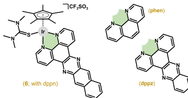
Fig. 2 Structural formulas of the complexes [\text{Ir}(\eta^5-\text{Cp}^*)(\text{dppn})(\text{tmtu})](\text{CF}_3\text{SO}_3)_2 ( 6 ), 1,10-phenanthroline (phen) and dipyrido [3,2- a :2',3'- c ]phenazine (dppz).
