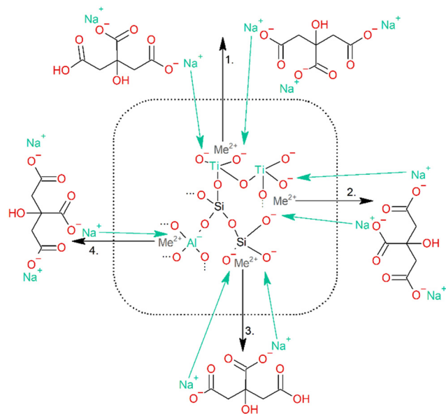
Fig. 15 Possible regeneration mechanism of \text{Me}^{2+} with di- and trisodium citrate species.
