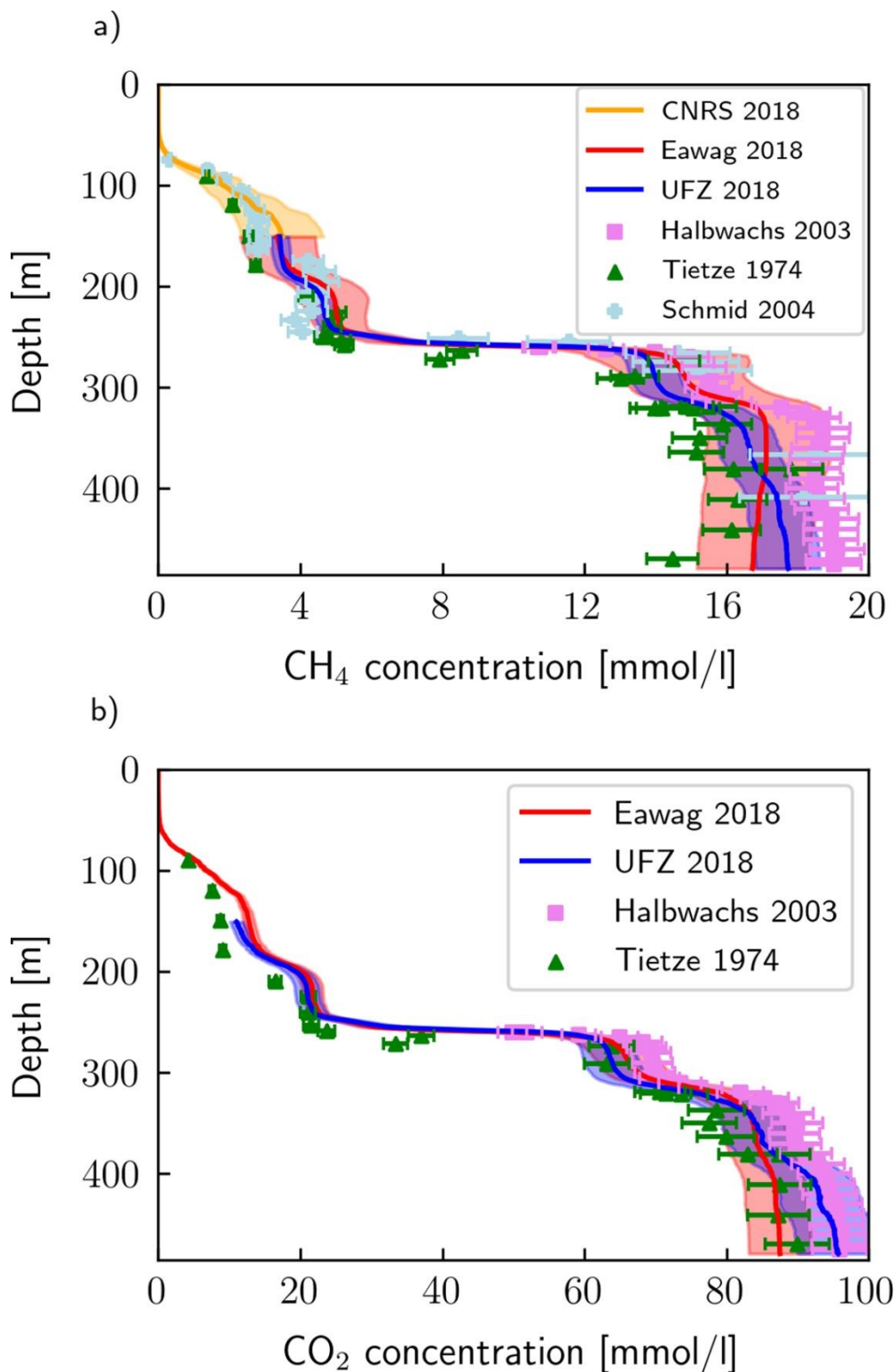
Fig. 3: Comparison between dissolved CH 4 and CO 2 concentrations measured by the 2018 campaign and those measured in 1974, 2003, and 2004. Reprinted (adapted) from reference 24. Copyright 2020 The Authors. 24
