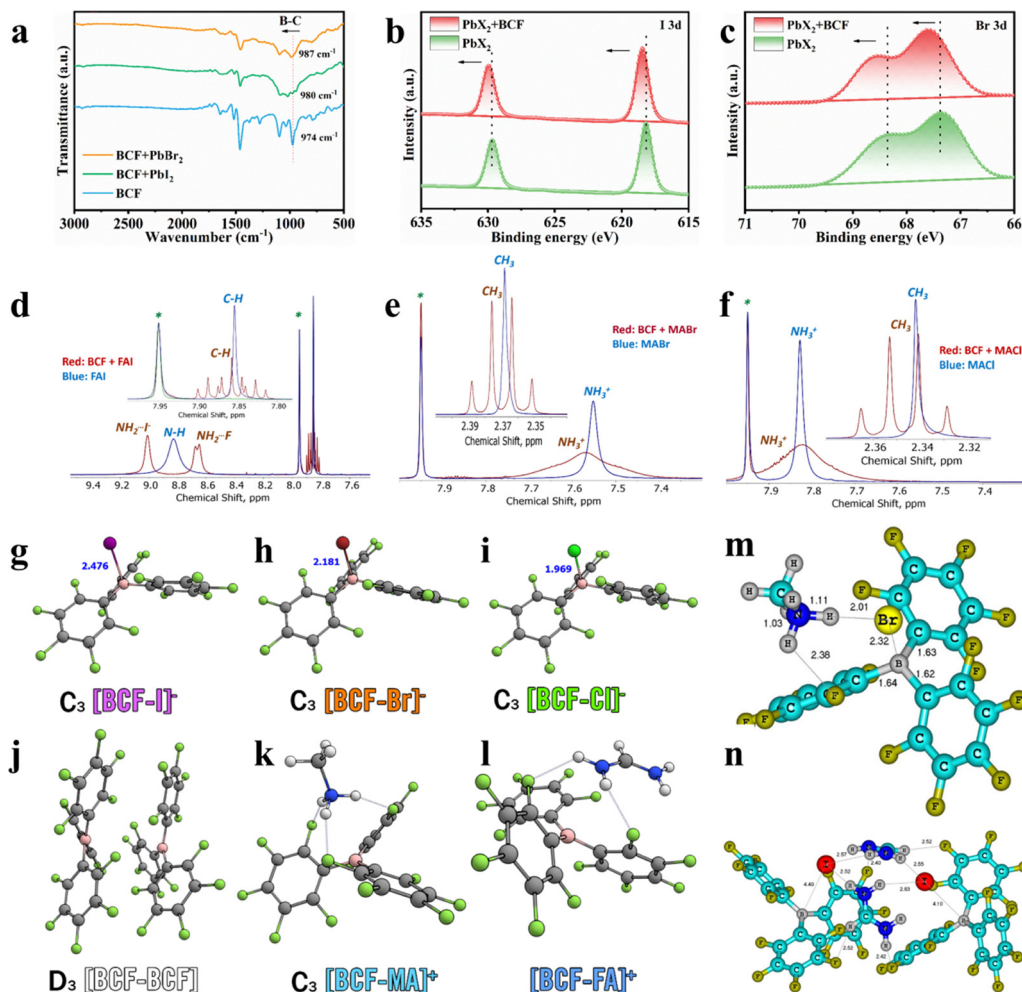
Fig. 1 FTIR spectra of (a) BCF and BCF + PbX 2 mixture. XPS spectra of (b) I 3d and (c) Br 3d for PbX 2 and PbX 2 + BCF films, respectively. The evolution of the 1 H NMR spectra of FAI (d), MABr (e) and MACl (f) upon interaction with BCF. The geometrical configuration of the [BCF-I] - (g), [BCF-Br] - (h), [BCF-Cl] - (i) anionic complexes. The [BCF-BCF] neutral dimer (j), and the [BCF-MA] + (k) and [BCF-FA] + (l) cationic complexes, where symmetry is present it is listed before the complex name. The computed minimal-energy molecular structures of the MABr + BCF (1:1, m) and FAI + BCF (2:2, n) complexes. Short contacts are shown in the figures.
