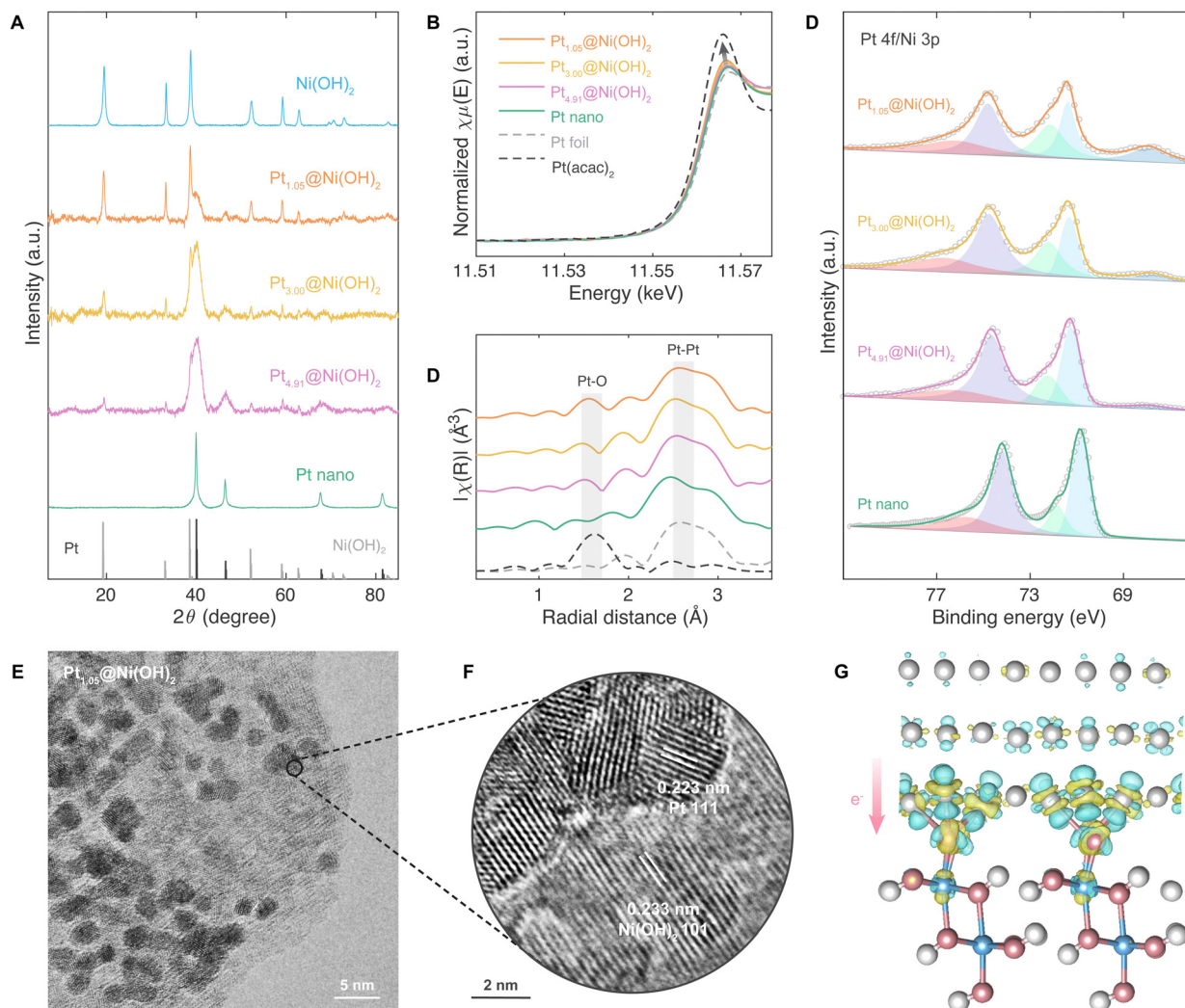
Fig. 1 Characterizations of \text{Pt}_x@Ni(OH)_2 ( x = 0.00, 1.05, 3.00, \text{ and } 4.91 ) and Pt nano. (a) XRD, (b) XANES, (c) EXAFS, and (d) XPS spectra for \text{Pt}_x@Ni(OH)_2 ( x = 0.00, 1.05, 3.00, \text{ and } 4.91 ) and Pt nano. (e) and (f) HRTEM images of \text{Pt}_{1.05}@Ni(OH)_2 . (g) Charge density difference of Pt–Ni(OH) 2 heterojunction. The cyan regions indicate charge depletion, while the yellow regions represent charge accumulation, with an isosurface value of 0.01 \text{ e} \text{ \AA}^{-3} .
