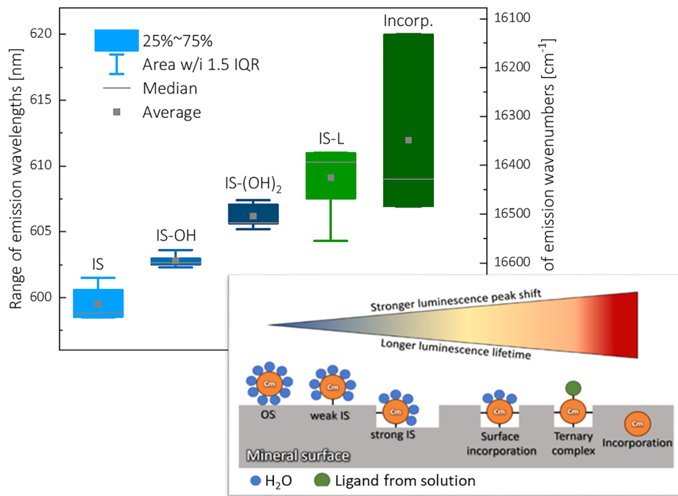
Fig. 3 Typical shift ranges for Cm III species found at the water/mineral interface. Bars show the interquartile range (IQR) and error bars 1.5 \times IQR, with median values represented as grey horizontal lines and average values as grey squares. The scheme at the bottom illustrates the species analyzed below and the general trends in peak shift and luminescence lifetime. Reprinted from Journal of Hazardous Materials, 423A, Demnitz, M. et al. , Effects of surface roughness and mineralogy on the sorption of Cm(III) on crystalline rock, 127006, Copyright (2022), with permission from Elsevier.
