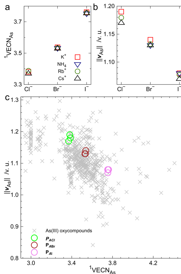
Fig. 11 Arsenic first-order valence entropy coordination number ( 1 VECN As ) and arsenic net bond valence vector length ( \|\mathbf{v}_{\text{As}}\| ), which equals the length of bond valence vector of arsenic lone electron pair, plotted as a function of the anion type present in the intercalates (a and b, respectively). 1 VECN As plotted as a function of \|\mathbf{v}_{\text{As}}\| for arsenic(III) oxycompounds (denoted with grey x markers) and for anhydrous hexagonal P AX intercalates denoted with colored circles (c). Data for arsenic(III) oxycompounds taken from ref. 38. Figure reprinted from M. Dąbrowski, W. Wrześniewska, A. Prystupiak, J. Zachara and P. A. Guńka, Cryst. Growth Des. , 2023, 23, 6081–6085. 39
