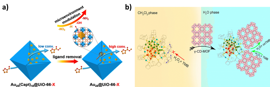
Fig. 8 (a) Schematic illustration showing the synthetic route to \text{Au}_{25}(\text{Capt})_{18}@\text{UiO-66-X} to surface clean \text{Au}_{25}@\text{UiO-66-X} for enhanced catalysis through microenvironment modulation around \text{Au}_{25} by adjusting the functional group on linker of MOF pore walls. Reproduced with permission from ref. 87. (b) Schematic illustration showing the encapsulation of \text{Au}_{40}(\text{S-Adm})_{22} by \gamma -CD-MOF to form \text{Au}_{40}/\gamma -CD-MOF for phase transfer and enhanced catalysis in horseradish peroxidase reaction. Reproduced with permission from ref. 88.
