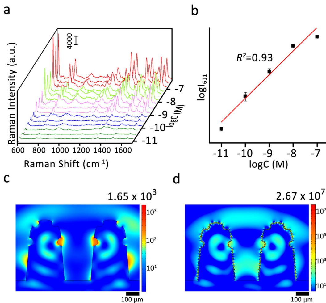
Fig. 5 (a) SERS activity of the substrate using the R6G solution with concentrations ranging from 10^{-7} to 10^{-11} M. (b) Correlation between the log–log plot of I_{611} and C_{\text{R6G}} . The error bar was obtained by three replicate determinations based on the Raman spectra in (a). (c) The electric field simulation of the C-NR substrate. (d) The electric field simulation of the C-NR@Ag substrate.
