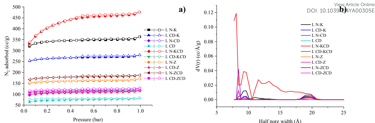
Figure 4. (a) N 2 adsorption/desorption isotherms of lignin-based activated porous carbons at -196 °C (solid symbols represent adsorption and hollow symbols indicates desorption), (b) pore size distribution from NLDFT method using N 2 isotherms at -196 °C.
