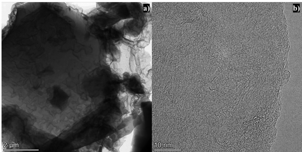
Figure 2. (a) Transmission electron micrograph and (b) High-resolution transmission electron micrograph of L N-K .
