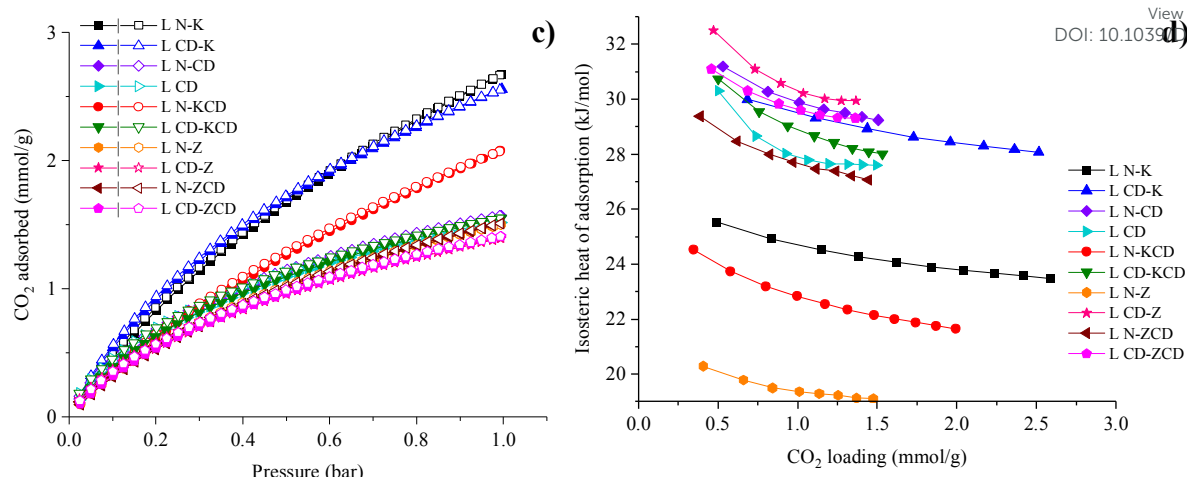
Figure 5. CO 2 adsorption isotherms at (a) 0 °C, (b) 25 °C, and (c) 40 °C (solid symbols represent adsorption, and hollow symbols indicate desorption), and (d) isosteric heat of CO 2 adsorption.
